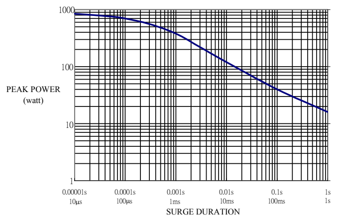
SURGE PERFORMANCE
