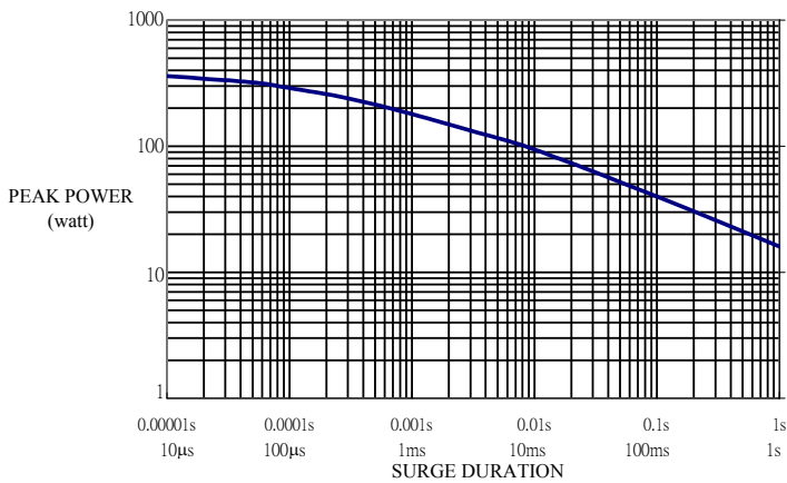
SURGE PERFORMANCE
